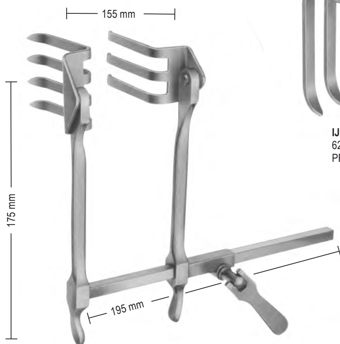
IJ-069 - IJ-072 SCOVILLE-RICHTER Retractor with 1 pair blades reversible type. The Retractor bar and shanks may be easily rotated 180 when blades are in situ.
