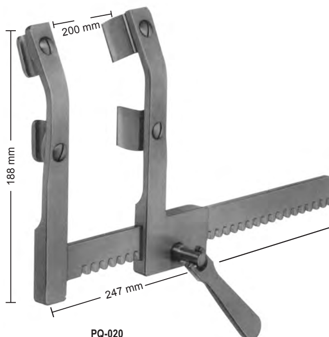
PQ-020 MORSE Sternotomy spreader for adults, with moveable double, each blade 19x19 mm
